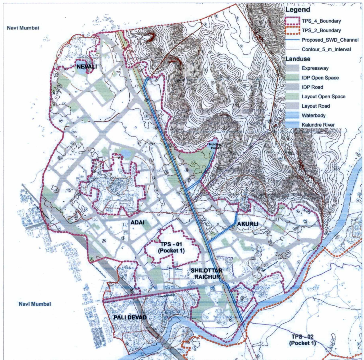
Figure 3: Proposed Storm Water Channel
