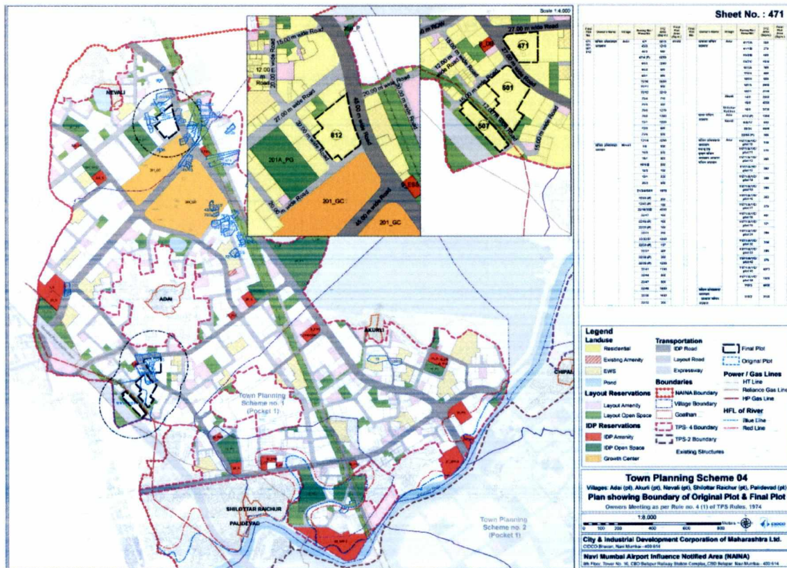
Figure 5: Plan Showing OP and FP in TPS layout
